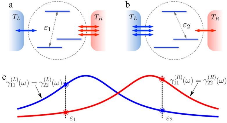
Fig. 4. (Color online) (a) Transition-1 couples more strongly to bath-R, \gamma_{11}^{(L)}(\varepsilon_1) < \gamma_{11}^{(R)}(\varepsilon_1) . (b) Transition-2 couples more strongly to bath-L, \gamma_{22}^{(L)}(\varepsilon_2) > \gamma_{22}^{(R)}(\varepsilon_2) . (c) An example of spectrums \gamma_{ii}^{(\omega)} to support such configurations of (a) and (b).
